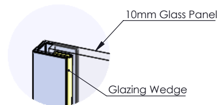
Glass To Wall Tolerance DETAIL A
