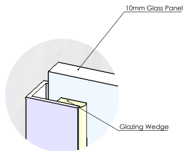
Glass To Wall Tolerance DETAIL A
