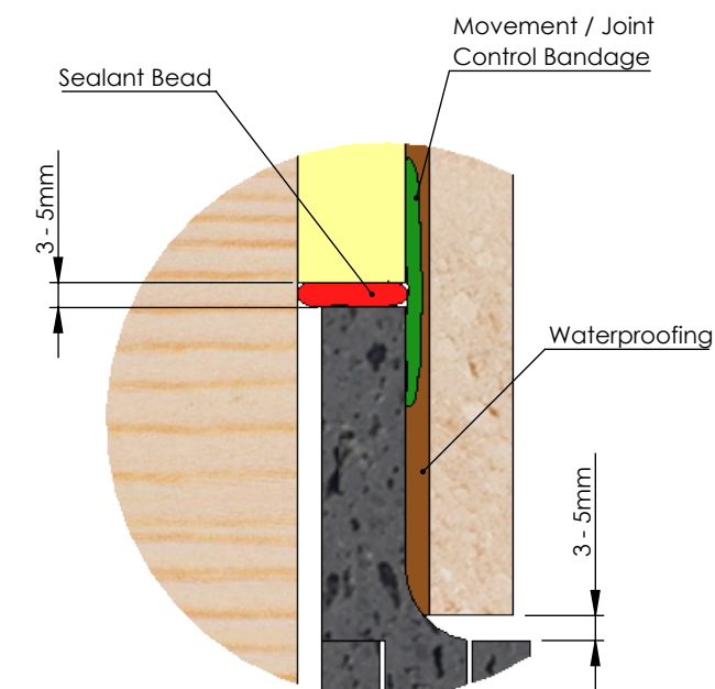
Wall Joint Detail DETAIL C
