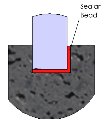
Glass Panel Silicone Detail
