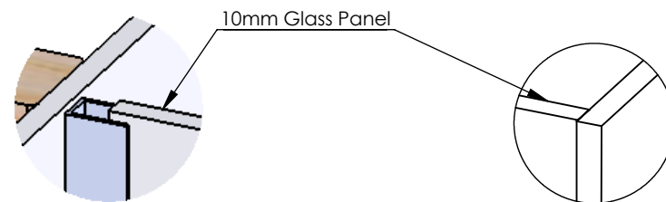
Corner Detail DETAIL B
