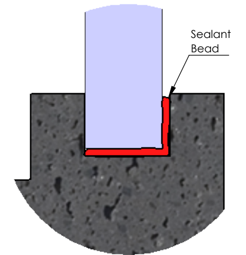
Glass Panel Silicone Detail DETAIL D
