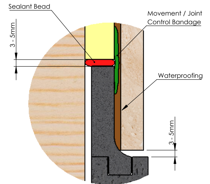
Wall Joint Detail DETAIL C
