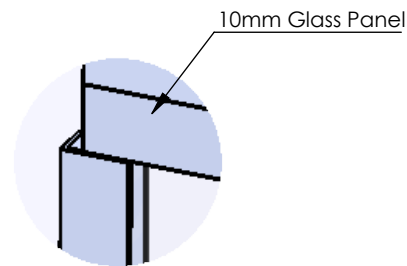
Glass To Wall Tolerance Rail Hidden DETAIL A
