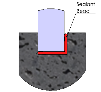
Glass Panel Silicone Detail
