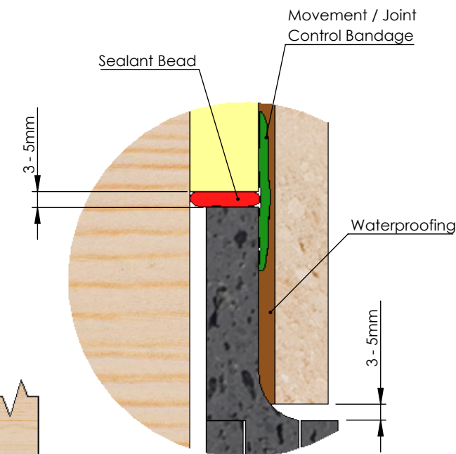
Wall Joint Detail DETAIL C
