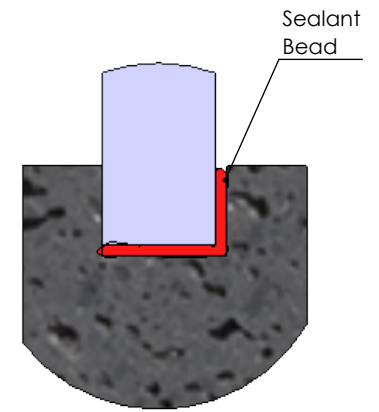
Glass Panel Silicone Detail
