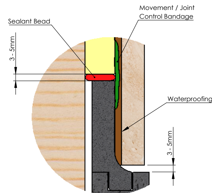
Wall Joint Detail DETAIL C
