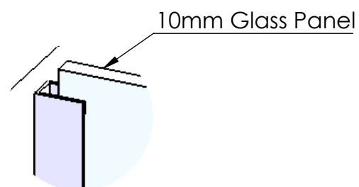
Glass To Wall Tolerance Rail Hidden DETAIL A
