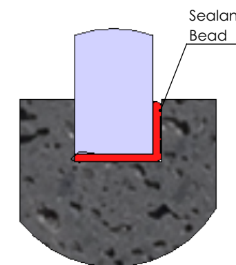
Glass Panel Silicone Detail
