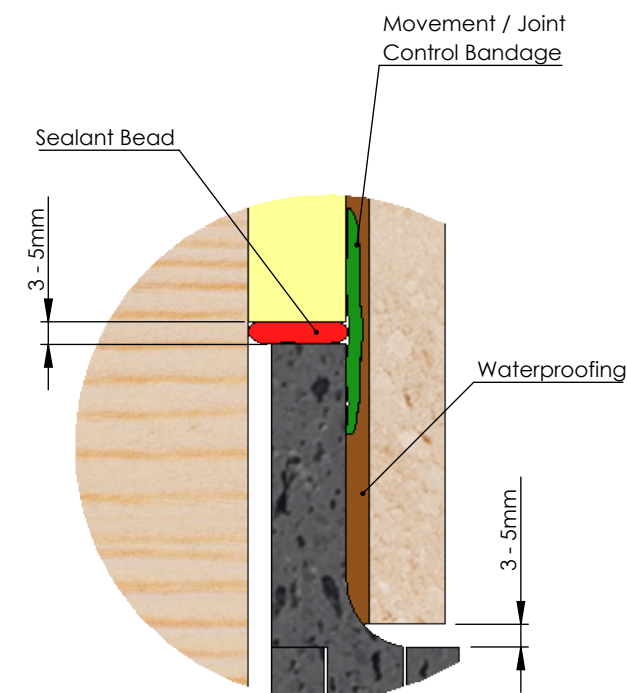
Wall Joint Detail DETAIL C
