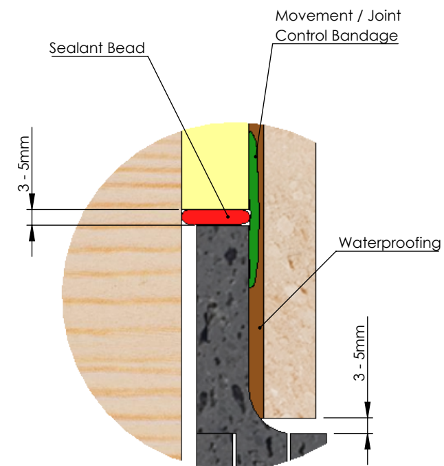
Wall Joint Detail DETAIL C
