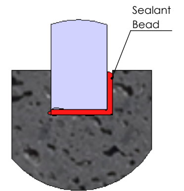
Glass Panel Silicone Detail
