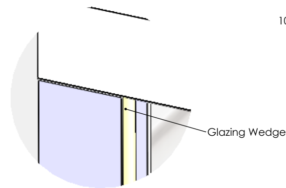
Glass To Wall Tolerance DETAIL A
